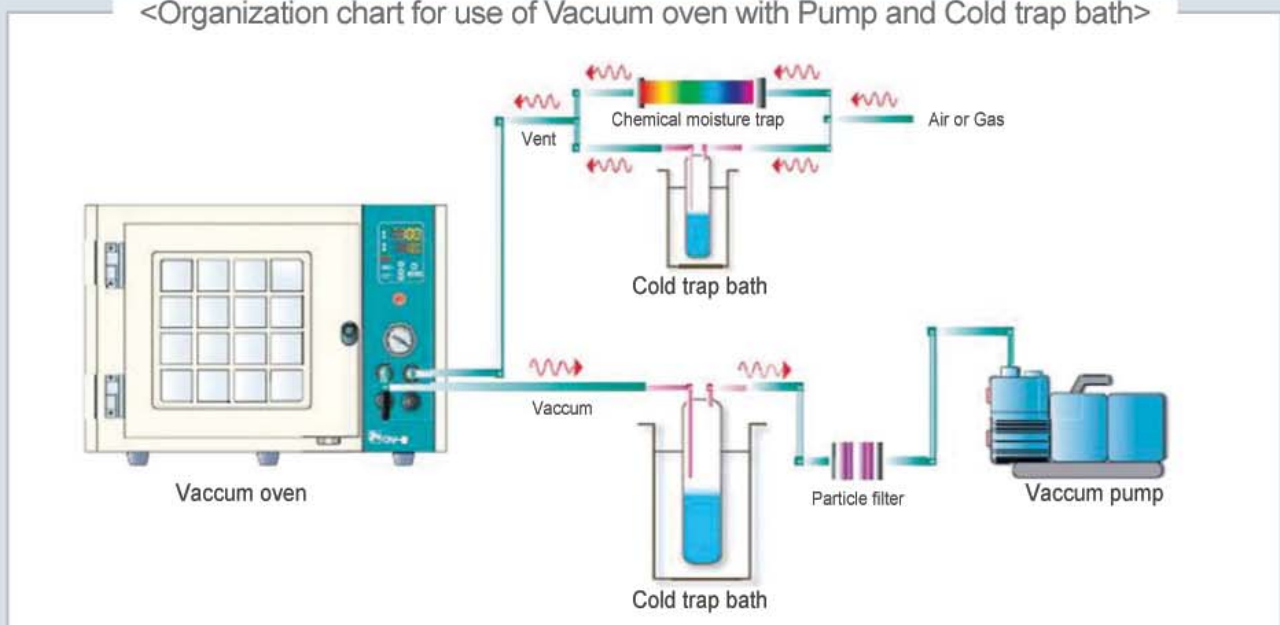
<Organization chart for use of Vacuum oven with Pump and Cold trap bath>
